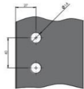
Glass drilling
